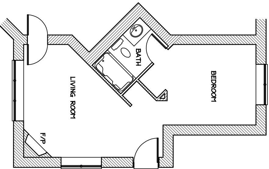
SANDPIPER 1 BEDROOM UNIT 450 SQ.FT.
